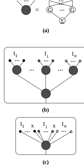
Fig. 5. (a): The basic HyperBF module; (b): A score-level integration network; (c): A feature-level integration network.
