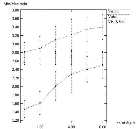
Fig. 7. Min/Max ratio of the FRS, SRS and integrated system (these last two are functions of the number of digits in the input speech signal); the spectral resolution of the SRS is 4; the vertical bars represent the standard deviation of the measured quantity.
