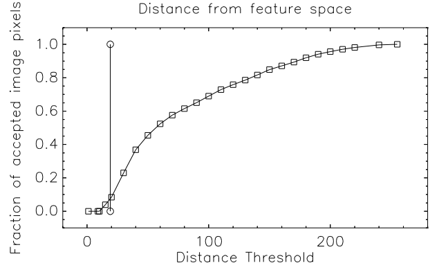
Fig. 12. The fraction of image pixels classified as right eye as a function of the threshold on the residual. The first 10 eigenvectors from a population of 60 images were used. The image used for the plot was of a person not in the database. The vertical line represent the threshold computed by summing the residual eigenvalues. The correct eye is the only selected region for d < 11 , the other eye being selected next.
