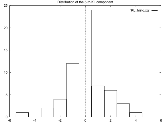
Fig. 13. The distribution of the values of the 5-th principal component computed from 60 eyes images. Note the clear unimodality of the distribution which suggests the effectiveness of using a quadratic classifier in the feature subspace. The other components present a similar distribution.
