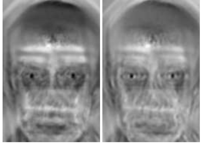
Fig. 7. The output of the correlation with an SDF computed using the spectral envelope of 20 training images as whitening preprocessing. Left: the normal SDF (20 examples). Right: a least square SDF with 6 templates (20 examples). The darker the image the higher the corresponding value. The least square SDF exhibits a sharper response using the same whitening filter.
