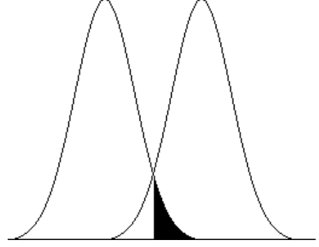
Fig. 1. The probability of error, represented by the shaded area, when the distributions are Gaussian with the same covariance.
