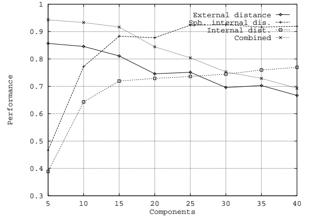
Fig. 17. Performance of different strategies based on the computation of principal components. The horizontal axis reports the number of components used in the expansion, while the vertical axis reports the percentage of eyes correctly located (see text for a detailed explanation).
